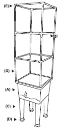
Assembly overview
